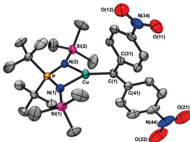
Figure 3. ORTEP diagram of the solid state structure of 4b . 50% ellipsoids, hydrogen atoms omitted for clarity. Selected bond lengths ( \text{\AA} ) and angles (deg): Cu–C(1) 1.8321(18), Cu–N(1) 1.9711(16), Cu–N(2) 1.9658(14), P–N(1) 1.6031(15); N(1)–P–N(2) 101.84(8), N(1)–Cu–N(2) 78.49(6), P–Cu–C(1) 175.68(6), N(2)–Cu–C(1)–C(31) 103.3(2), N(2)–Cu–C(1)–C(41) -83.8(2) .
